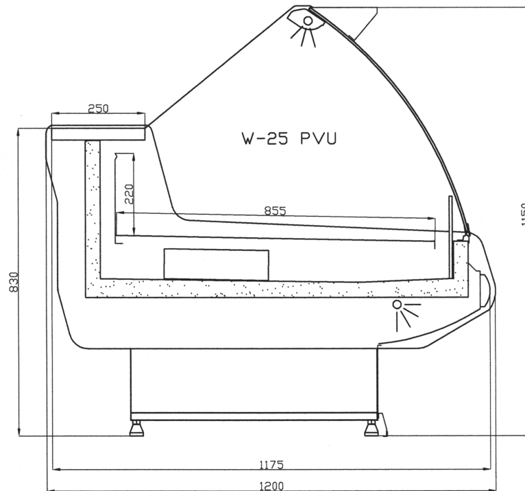
Refrigerated display case "W-PVU" – depth: 1200 mm
