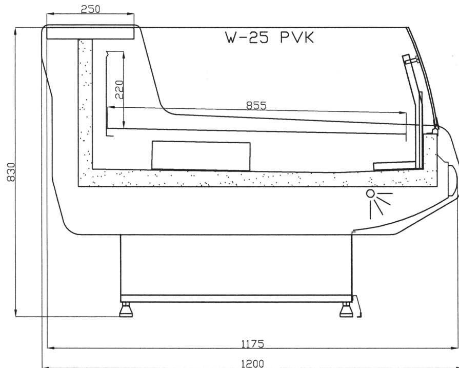
Refrigerated display case "W-PVK" - depth 1200 mm, height 830 mm
